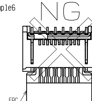
- Incorrect assembled - (Insufficiently inserted)
