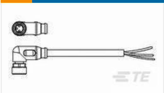
TE Part #2273009-1 M8 x 1.0 Angled socket Pigtail
