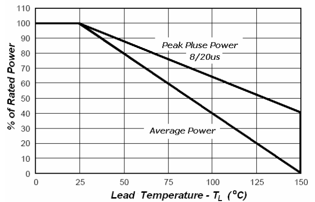
Fig 2. Power Derating
