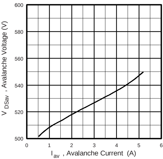
Fig. 12d - Typical Drain-to Source Voltage vs. Avalanche Current
