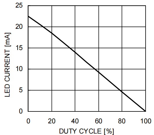
LED Current vs. Duty Cycle
