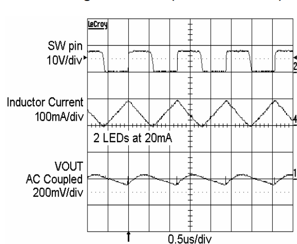
Switching Waveforms (2 LEDs in Series)
