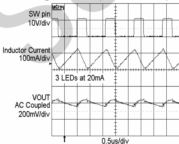
Switching Waveforms (3 LEDs in Series)
