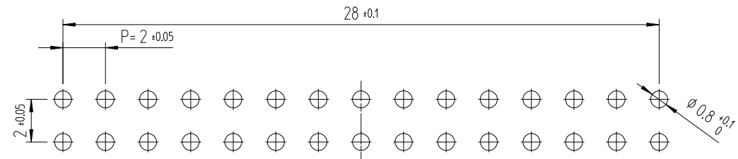
RECOMMENDED LAND PATTERN (FREE) (PCB THICKNESS t=1.6mm)
