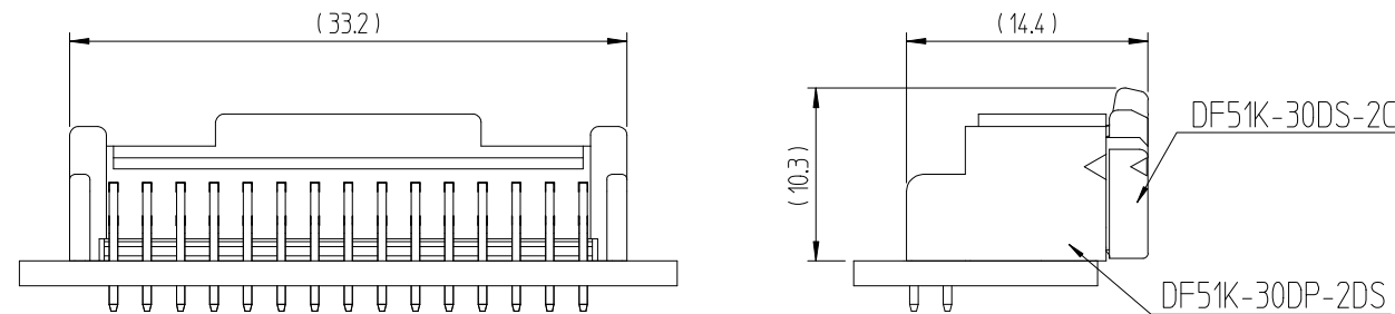
ENGAGEMENT FIGURE (2:1)
