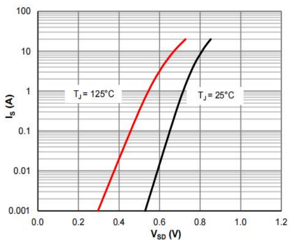
Figure 7: Body-Diode Characteristics
