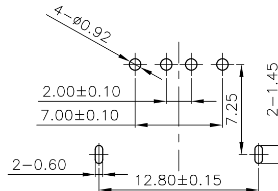
FRONT EDGE OF CONNECTOR PCB LAYOUT
