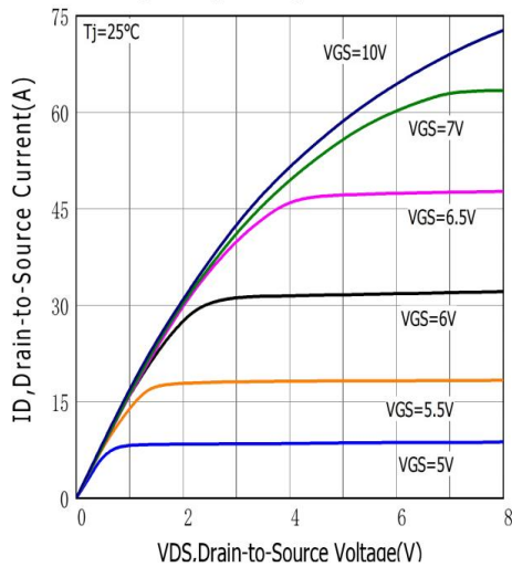
Figure.1 Typical Output Characteristics
