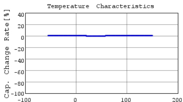
RHE5G2A272J1DBH03A C-Temp. capchange, DC0V,
