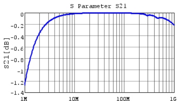
RHE5G2A272J1DBH03A S21 DC0V, 25degC
