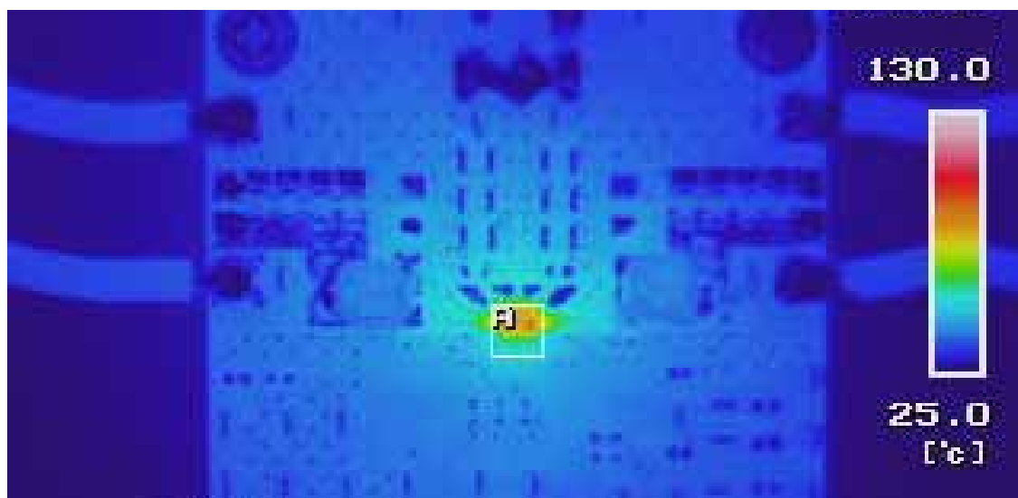
Figure 10-1 : Thermal image
