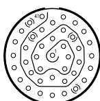
20-41 41 Size 20 Contacts
