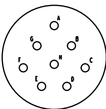
17-08 8 Size 16 Contacts
