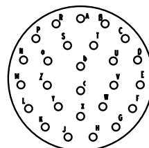
17-26 26 Size 20 Contacts
