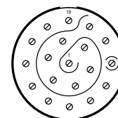
22-19 19 Size 16 Contacts
