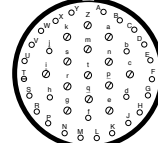
22-41 27 Size 20 Contacts 14 Size 16 Contacts
