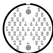
61-5 49 Size 20 Contacts 2 Size 8 Contacts *
