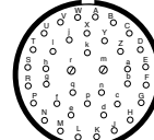
20-39 37 Size 20 Contacts 2 Size 16 Contacts
