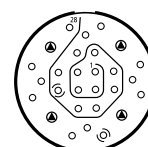
20-28 24 Size 20 Contacts 4 Size 12 Contacts
