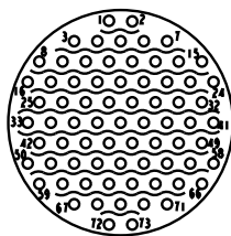
17-23 73 Size 23 Contacts
