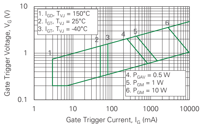
Figure 4. Gate Trigger Voltage vs. Gate Trigger Current
