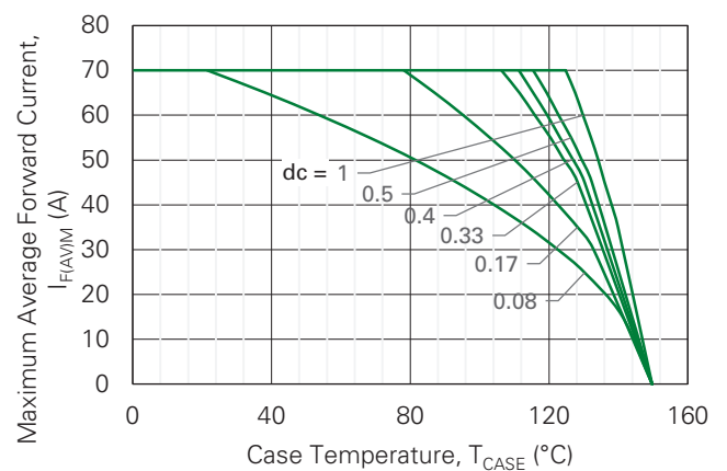
Figure 6. Max. Forward Current vs. Case Temperature
