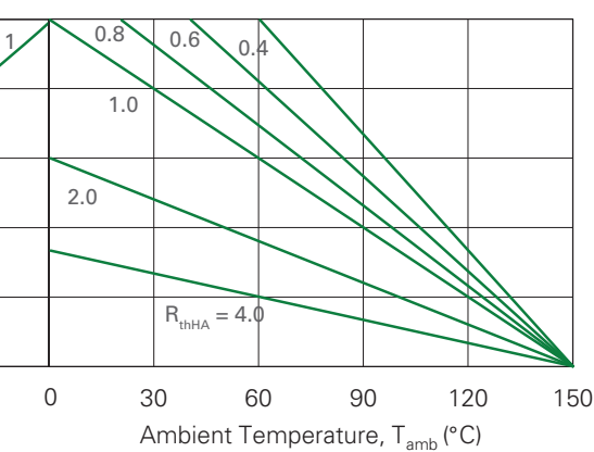
Figure 7b. Power Dissipation vs. Ambient Temperature
