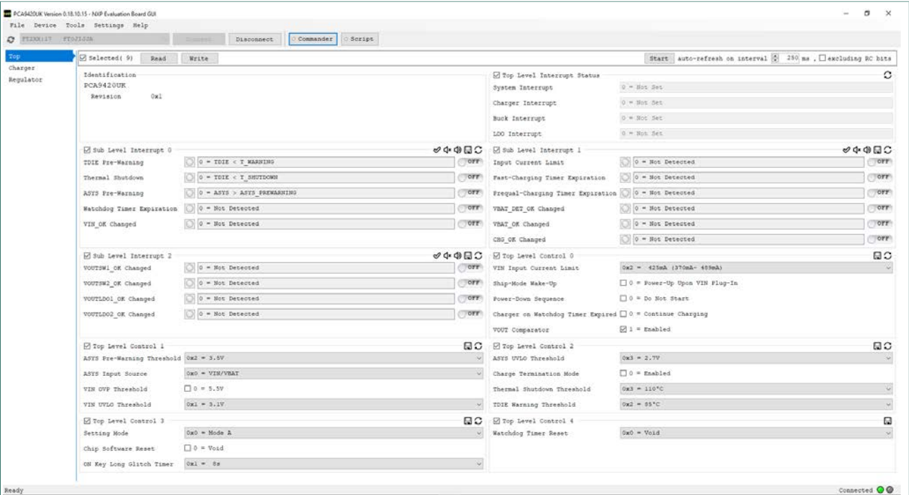
Figure 6. GUI overview
