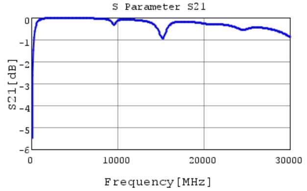
GJM0335C1H100JB01 S21 DCOV, 25degC
