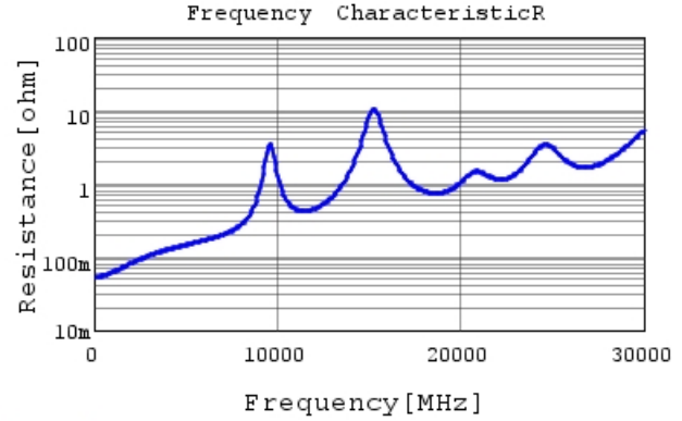
GJM0335C1H100JB01 R DCOV, 25degC
