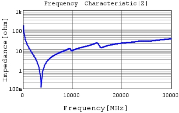
GJM0335C1H100JB01 |Z| DCOV, 25degC
