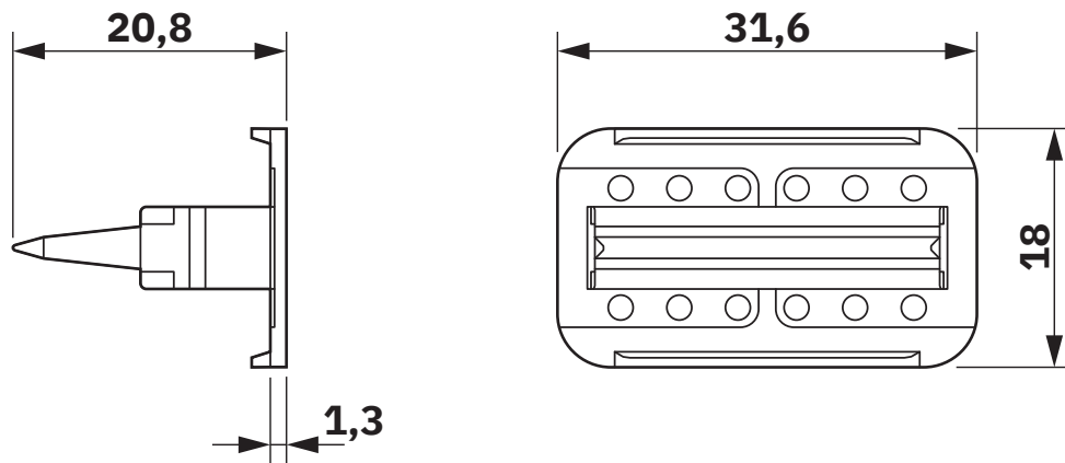
AW12S top view and side view
