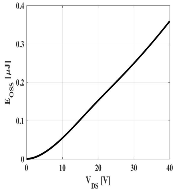
Figure 17: CossStored Energy
