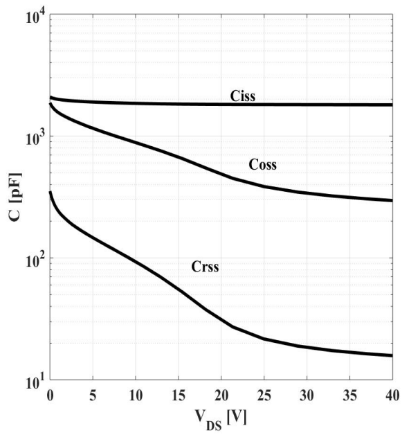
Figure 16: Typ. Capacitances
