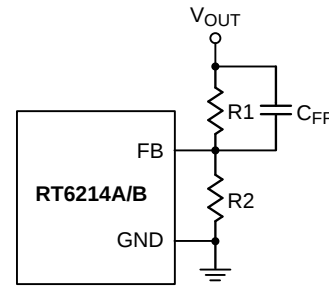
Figure 1. C_{\text{FF}} Capacitor Setting
