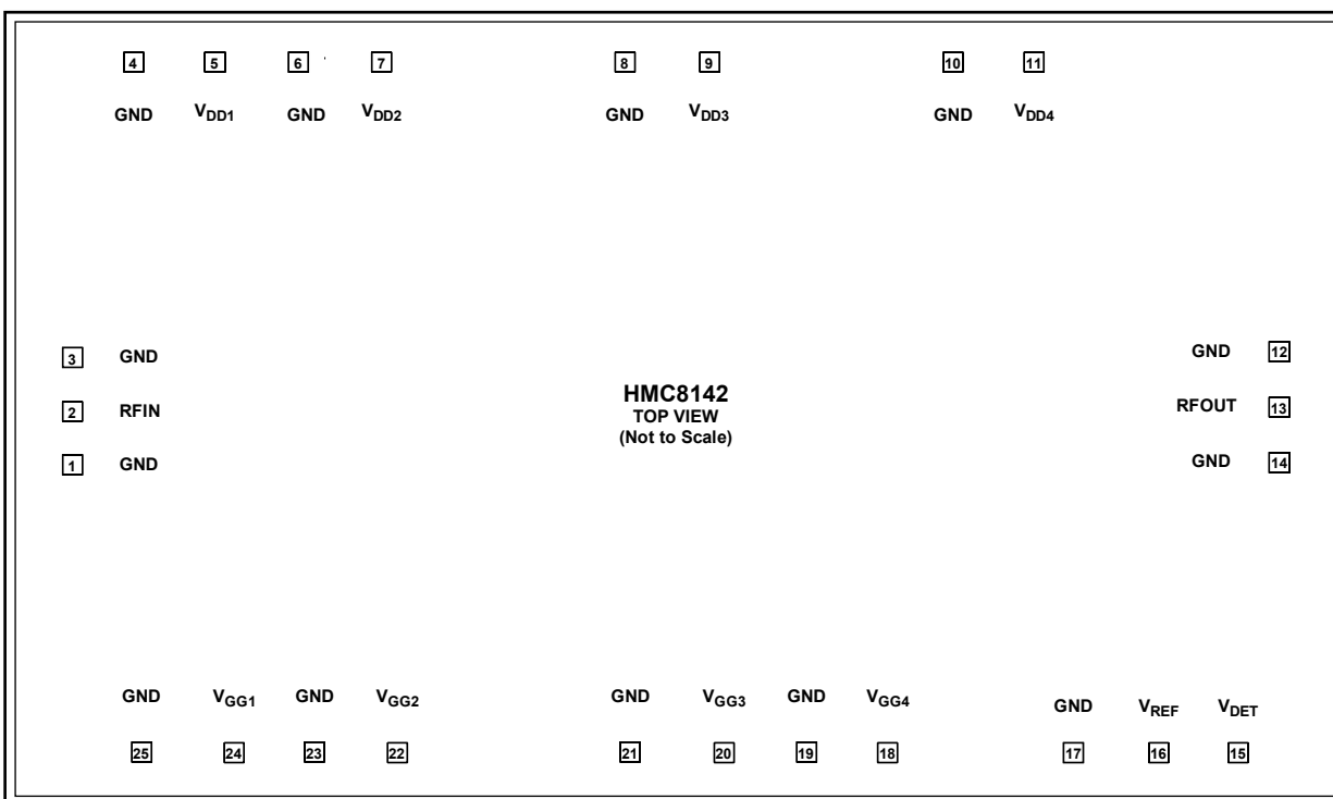
Figure 2. Pad Configuration
