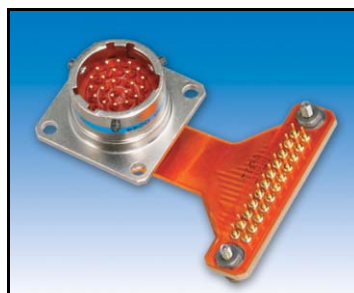
Flex Circuitry for Attachment to Printed Circuit Boards
