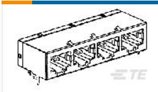
TE Part #5558524-1 MJ,1X4,R/A,8P,PNL GND,CAT5 NT
