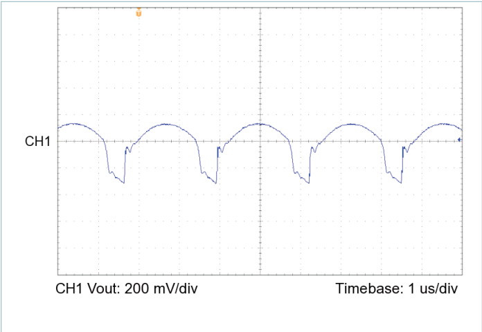
Figure 16 — Output voltage ripple, V_{IN} = 28\text{ V} , V_{OUT} = 3.3\text{ V} , C_{OUT\_EXT} = 1000\text{ }\mu\text{F} , R_{LOAD} = 0.091\text{ }\Omega
