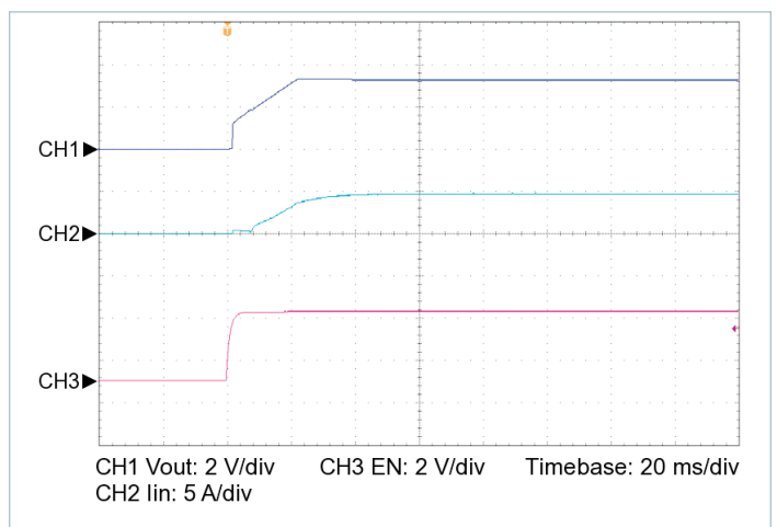
Figure 14 — Startup from EN, V_{IN} = 28\text{ V} , C_{OUT\_EXT} = 20000\text{ }\mu\text{F} , R_{LOAD} = 0.091\text{ }\Omega
