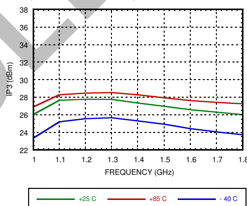
Output IP3 vs. Temperature [2]
