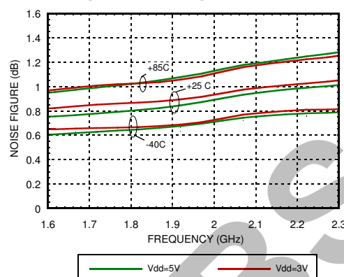
Noise Figure vs Temperature [1] [2] [3]
