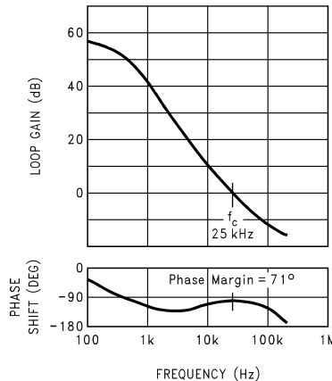
Figure 24. Measured Gain/Phase Plot for 3.3V/4A Application
