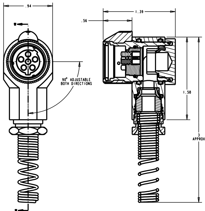
SECTION W-W
