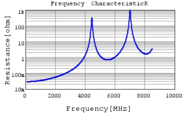
GQM22M5C2H120GB01 R DCOV, 25degC
