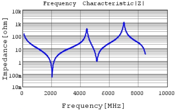
GQM22M5C2H120GB01 |Z| DCOV, 25degC
