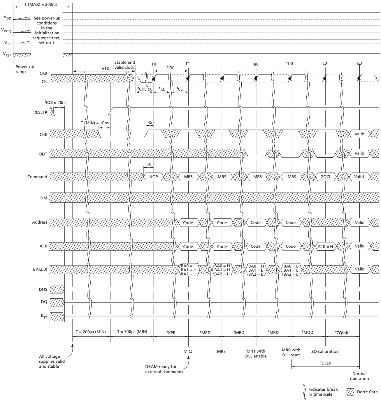
Figure 45: Initialization Sequence
