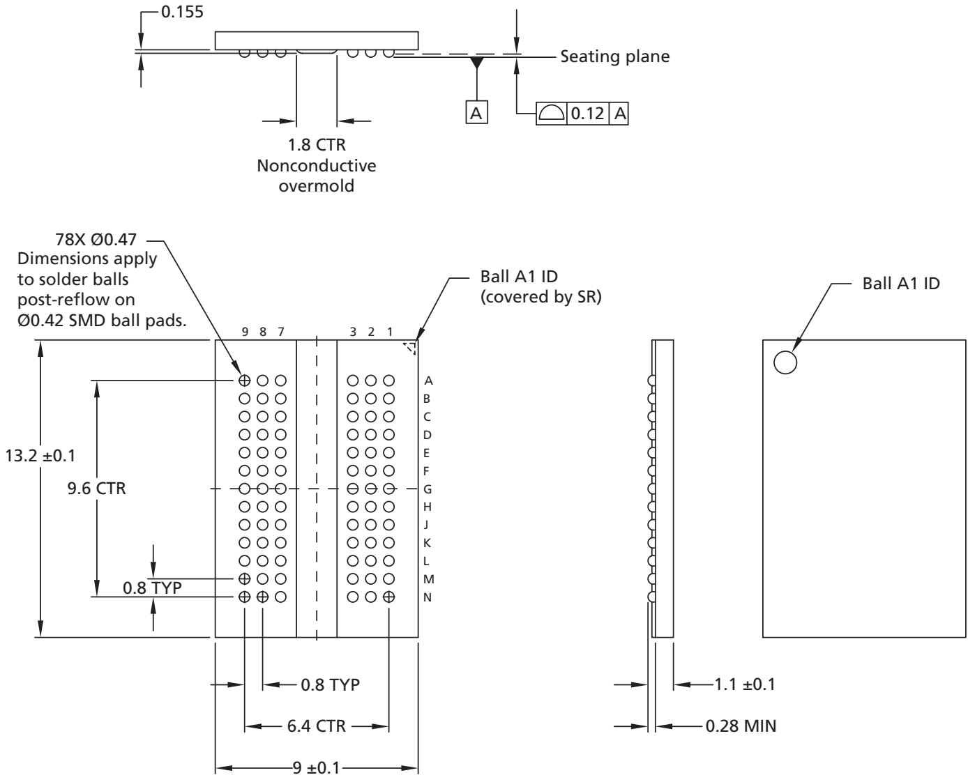
Figure 7: 78-Ball FBGA – x4, x8 (SN)
