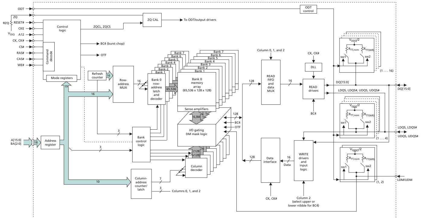
Figure 4: 512 Meg x 16 Functional Block Diagram
