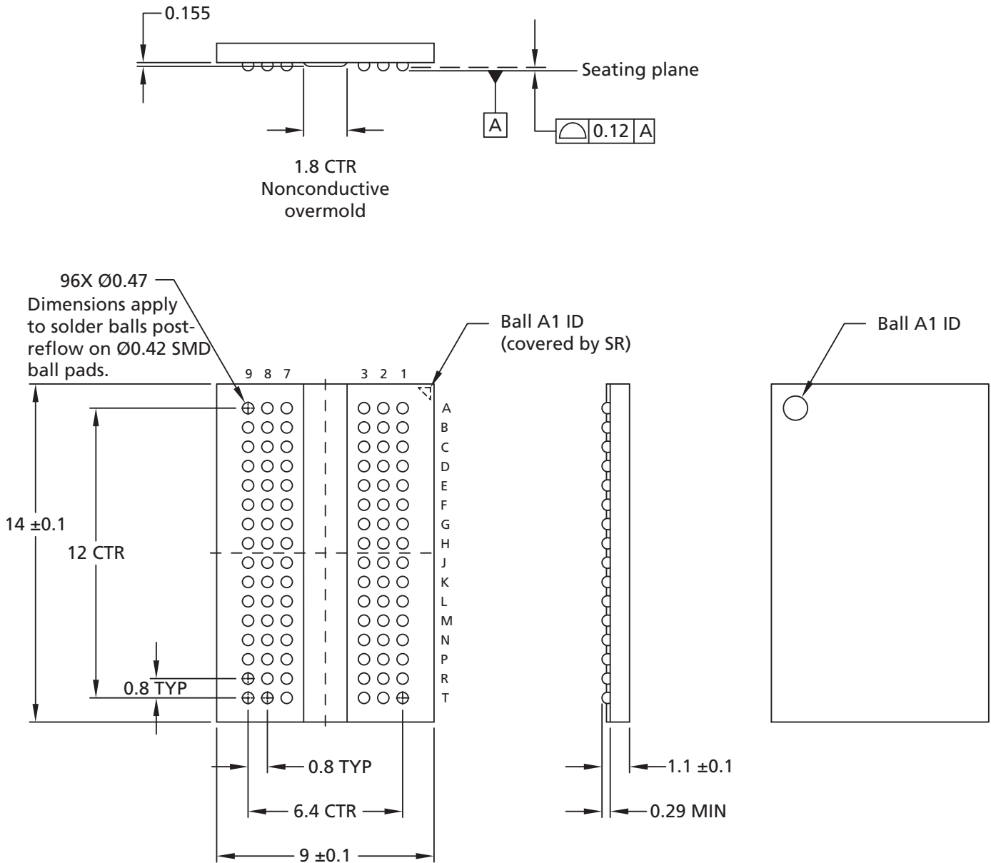
Figure 8: 96-Ball FBGA – x16 (HA)
