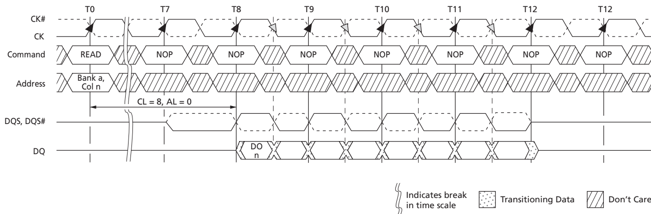
Figure 64: READ Latency
