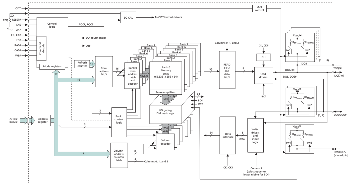
Figure 3: 1 Gig x 8 Functional Block Diagram
