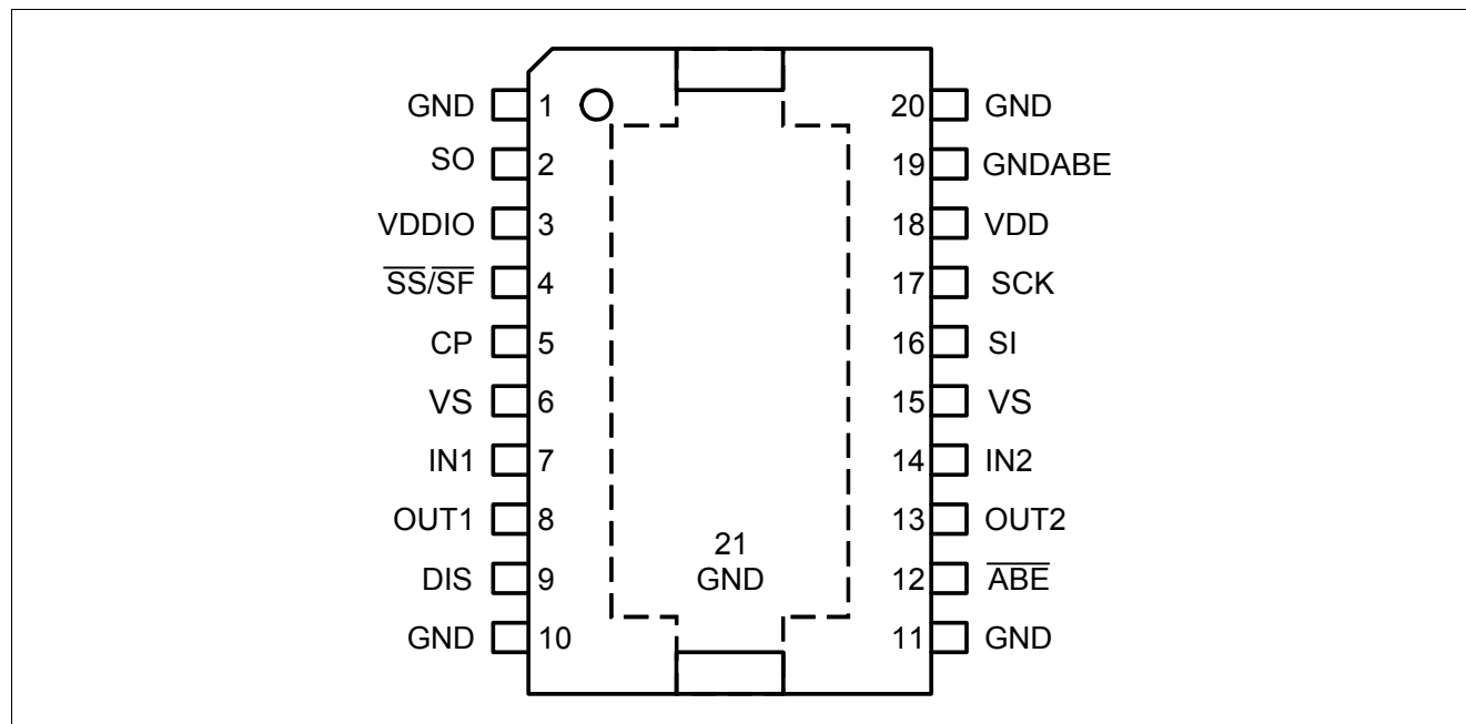
Figure 1 Pinout TLE8209-4SA
