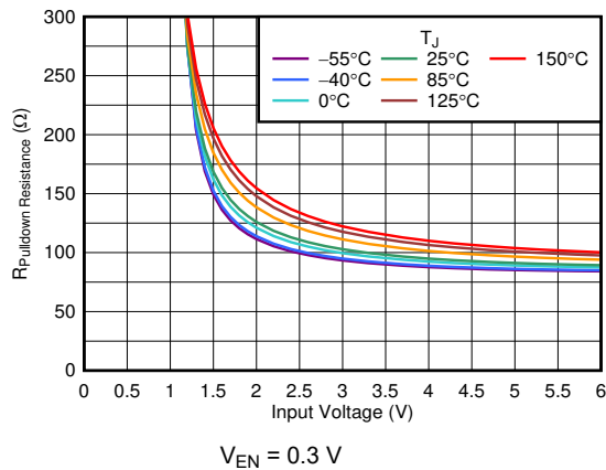
Figure 6-19. Pulldown Resistor ( R_{Pulldown} ) vs V_{IN}
