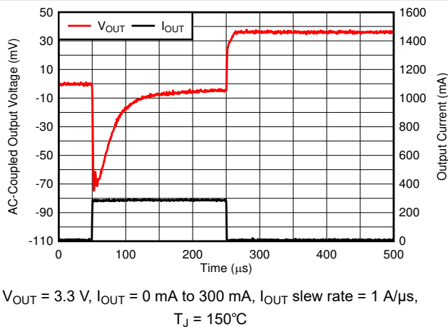
Figure 6-61. Load Transient
