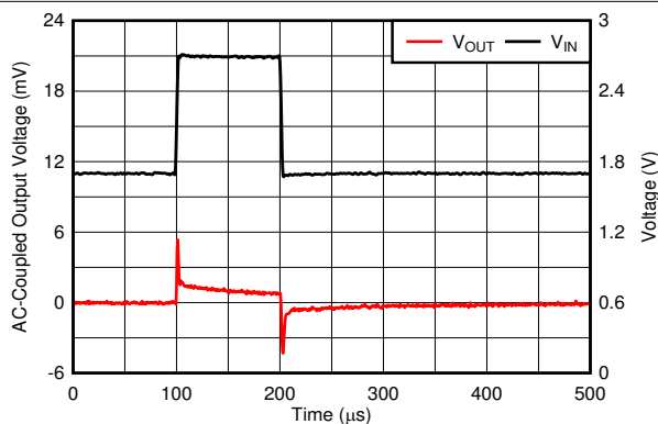
Figure 6-28. Line Transient
