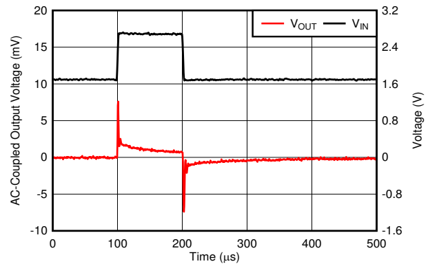
Figure 6-32. Line Transient
