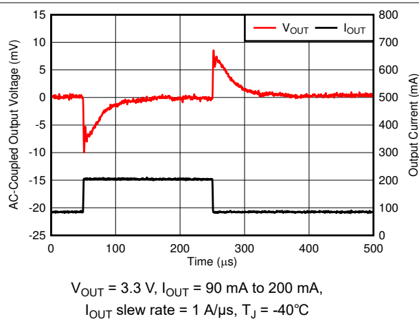
Figure 6-63. Load Transient
