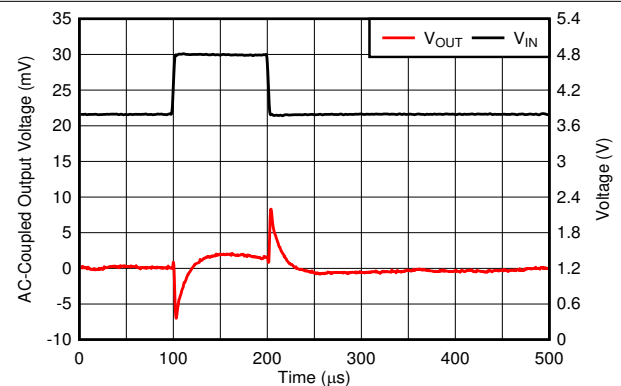
Figure 6-34. Line Transient
