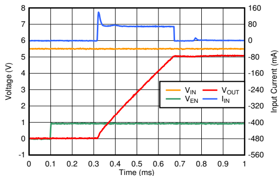
Figure 6-75. Start-Up Inrush Current With C_{OUT} = 1\text{ }\mu\text{F}
