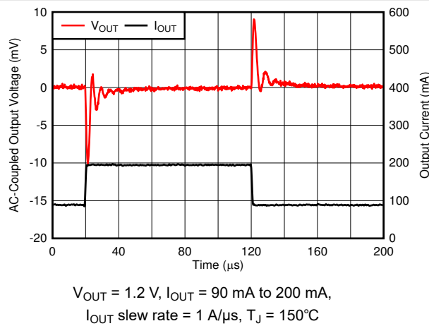
Figure 6-55. Load Transient
