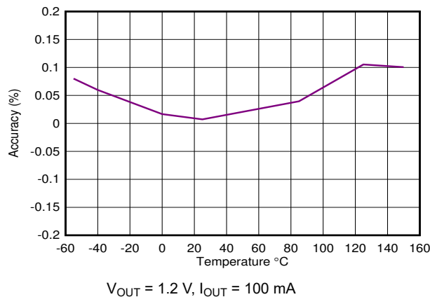
Figure 6-9. Accuracy vs Temperature
