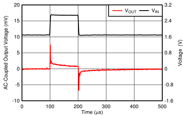
Figure 6-31. Line Transient
