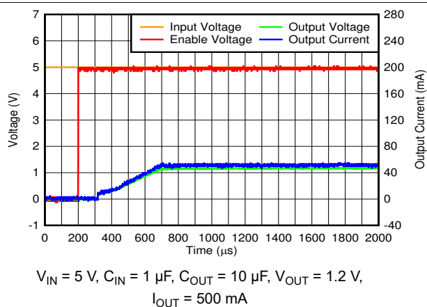
Figure 6-80. Start Up at 150^\circ\text{C}
