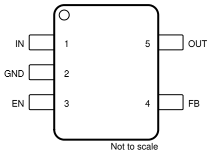
Figure 5-3. DBV Package (Adjustable), 5-Pin SOT-23, Top View
