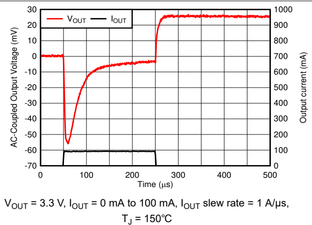
Figure 6-58. Load Transient
