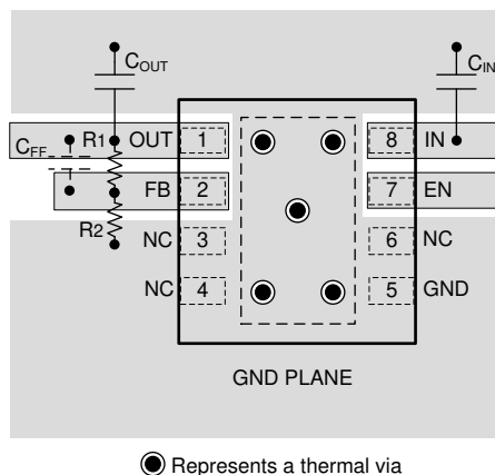
Figure 10-5. Layout Example for the DRB Package Adjustable Version
