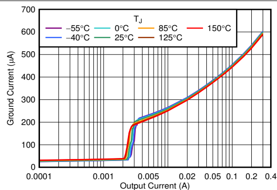
Figure 6-14. I_{GND} vs I_{OUT}
