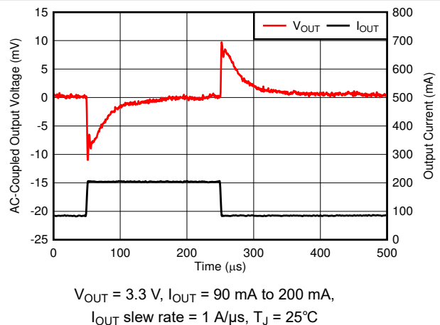
Figure 6-62. Load Transient
