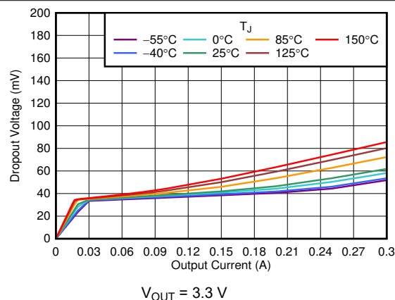
Figure 6-12. Dropout Voltage vs I_{OUT}
