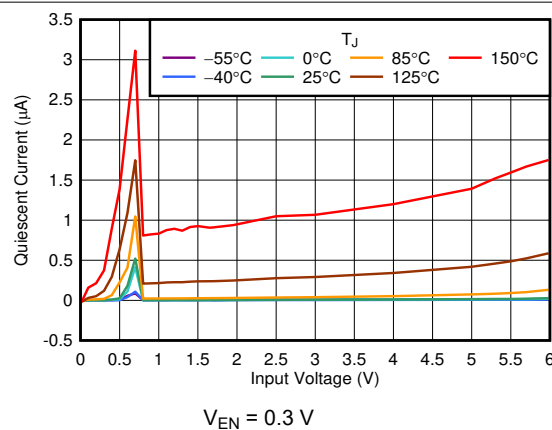
Figure 6-18. I_{SHDN} vs V_{IN}
