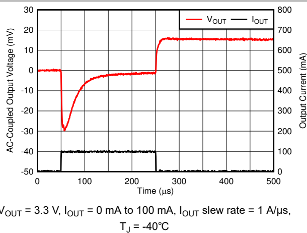
Figure 6-57. Load Transient
