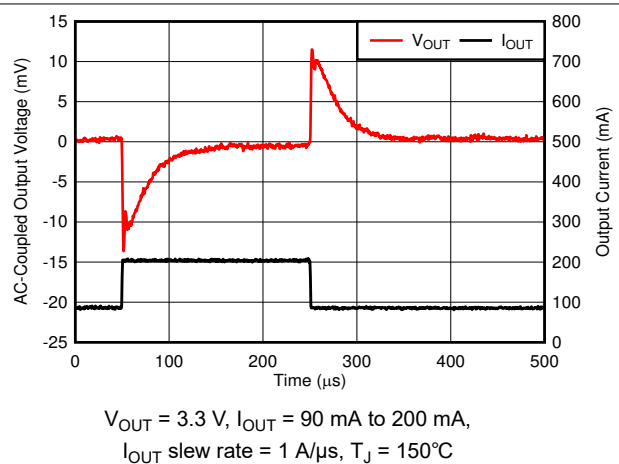
Figure 6-64. Load Transient
