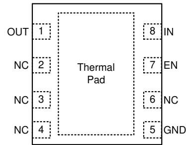
Figure 5-2. DRB Package (Fixed), 8-Pin VSON, Top View
