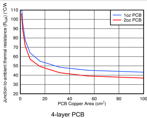
Figure 10-1. Junction-to-Ambient Thermal Resistance ( R_{JA} ) vs PCB Copper Area
