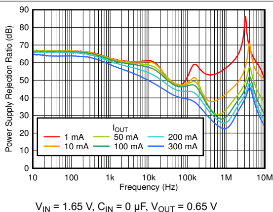
Figure 6-65. PSRR vs Frequency and I_{OUT}
