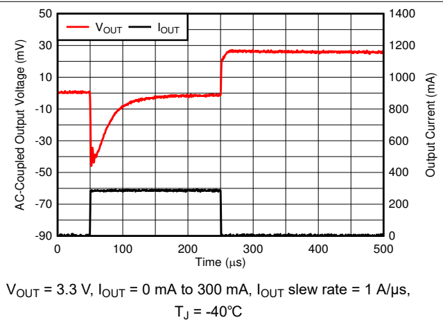
Figure 6-60. Load Transient
