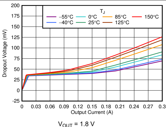
Figure 6-11. Dropout Voltage vs I_{OUT}
