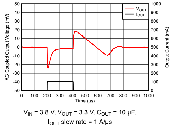
Figure 8-10. I_{OUT} Transient From 1 mA to 100 mA
