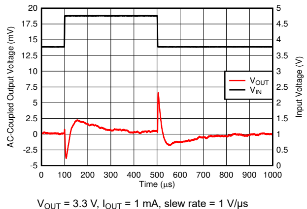
Figure 6-24. Line Transient
