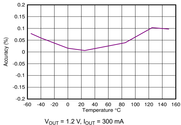
Figure 6-10. Accuracy vs Temperature
