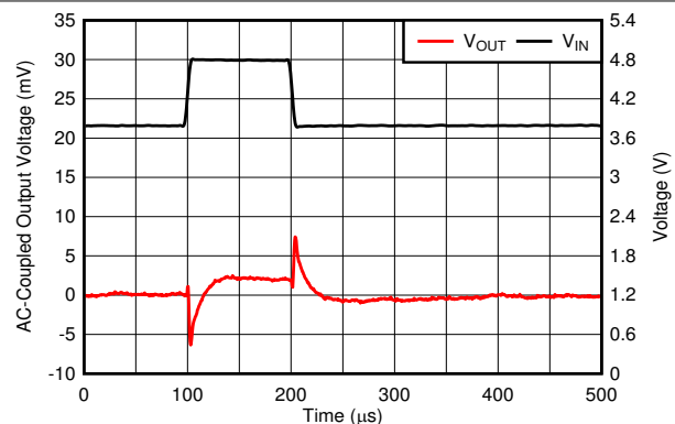
Figure 6-38. Line Transient
