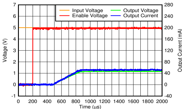
Figure 6-76. Start-Up Inrush Current With C_{OUT} = 1\text{ }\mu\text{F}
