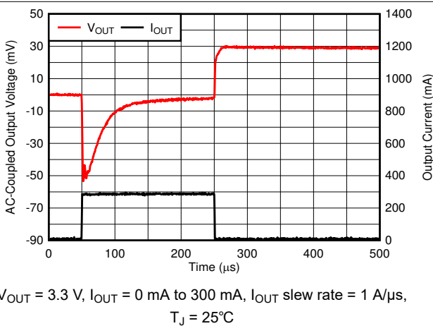
Figure 6-59. Load Transient
