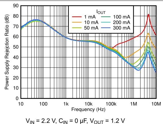
Figure 6-66. PSRR vs Frequency and I_{OUT}
