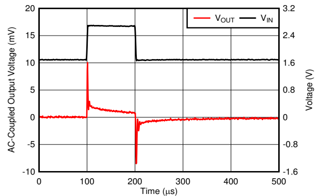
Figure 6-32. Line Transient
