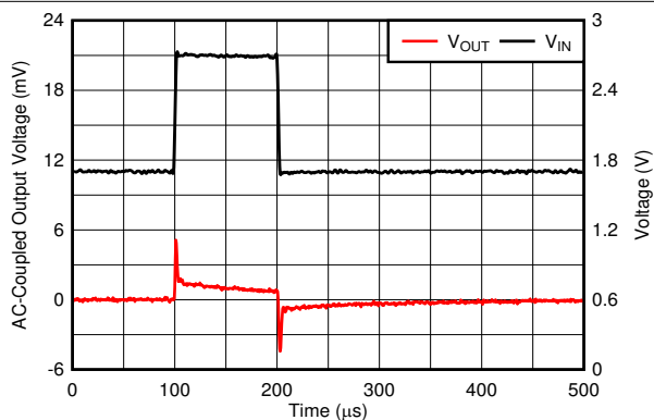
Figure 6-27. Line Transient
