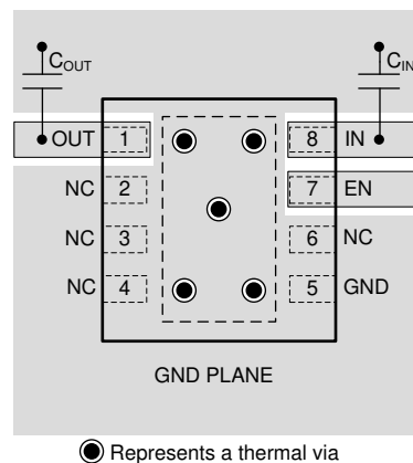
Figure 10-6. Layout Example for the DRB Package Fixed Version
