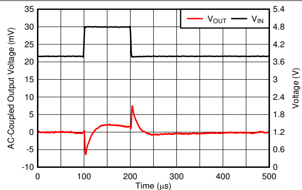
Figure 6-33. Line Transient
