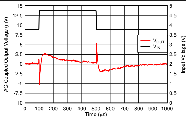
Figure 6-25. Line Transient
