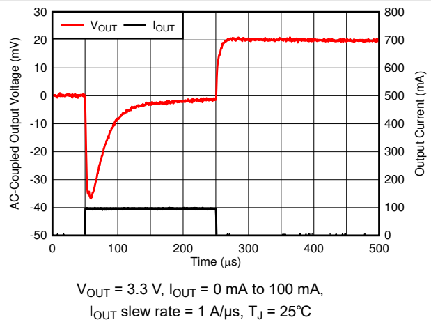
Figure 6-56. Load Transient
