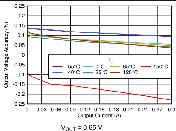
Figure 6-1. Output Accuracy vs I_{\text{OUT}}
