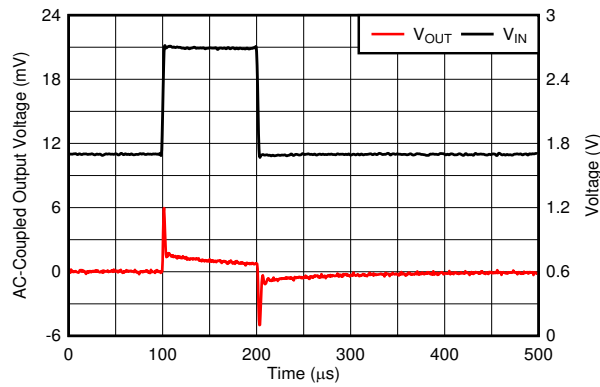
Figure 6-31. Line Transient
