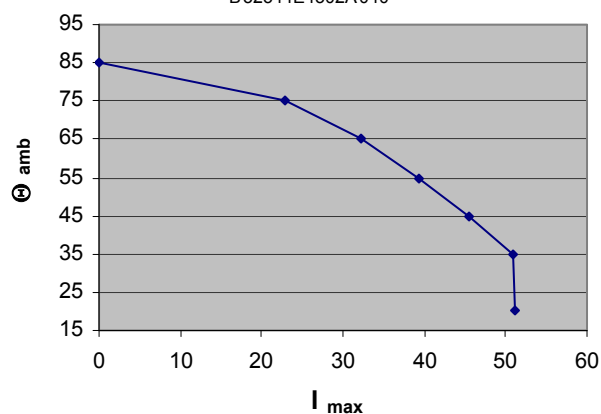
Max. allowable ambient Temp. at specific current (rms) B32344E4302A040
