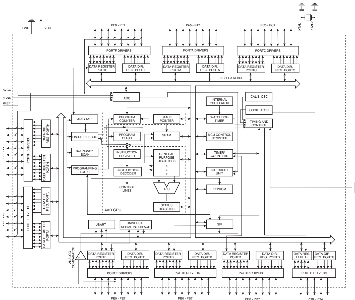
Figure 2-1. Block diagram.
