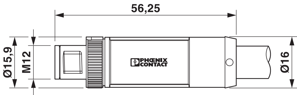
Dimensional drawing
