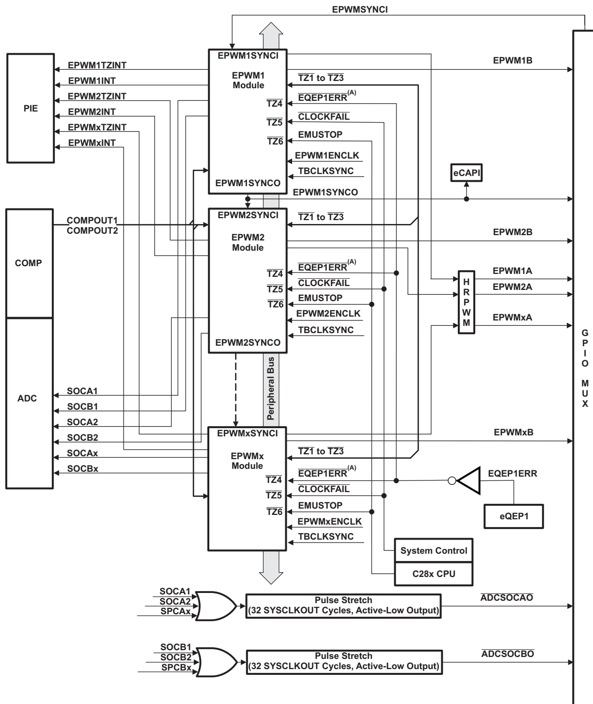
Figure 5-42. ePWM
