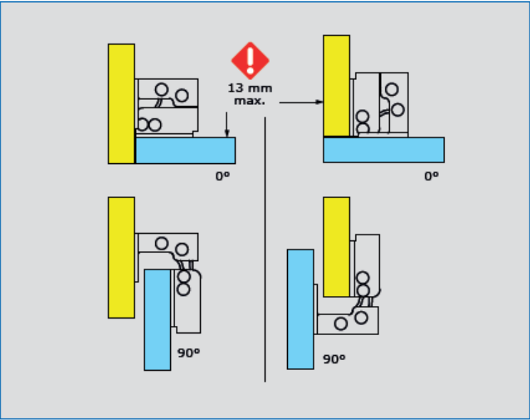
Nested door assembly shown Surface mounted assembly shown
