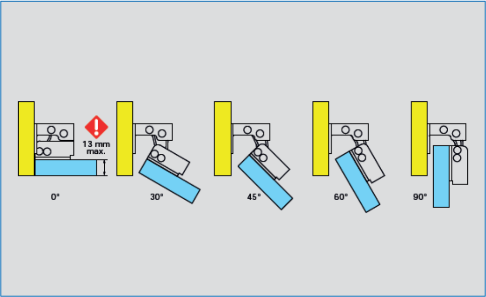
Nested door assembly shown
