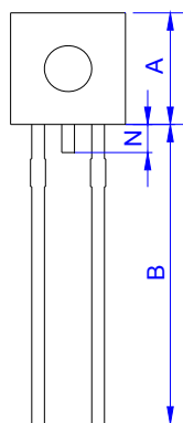
TO-92-2L
