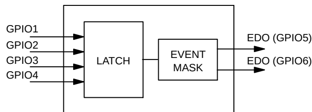
Figure 84. EDO Circuit
