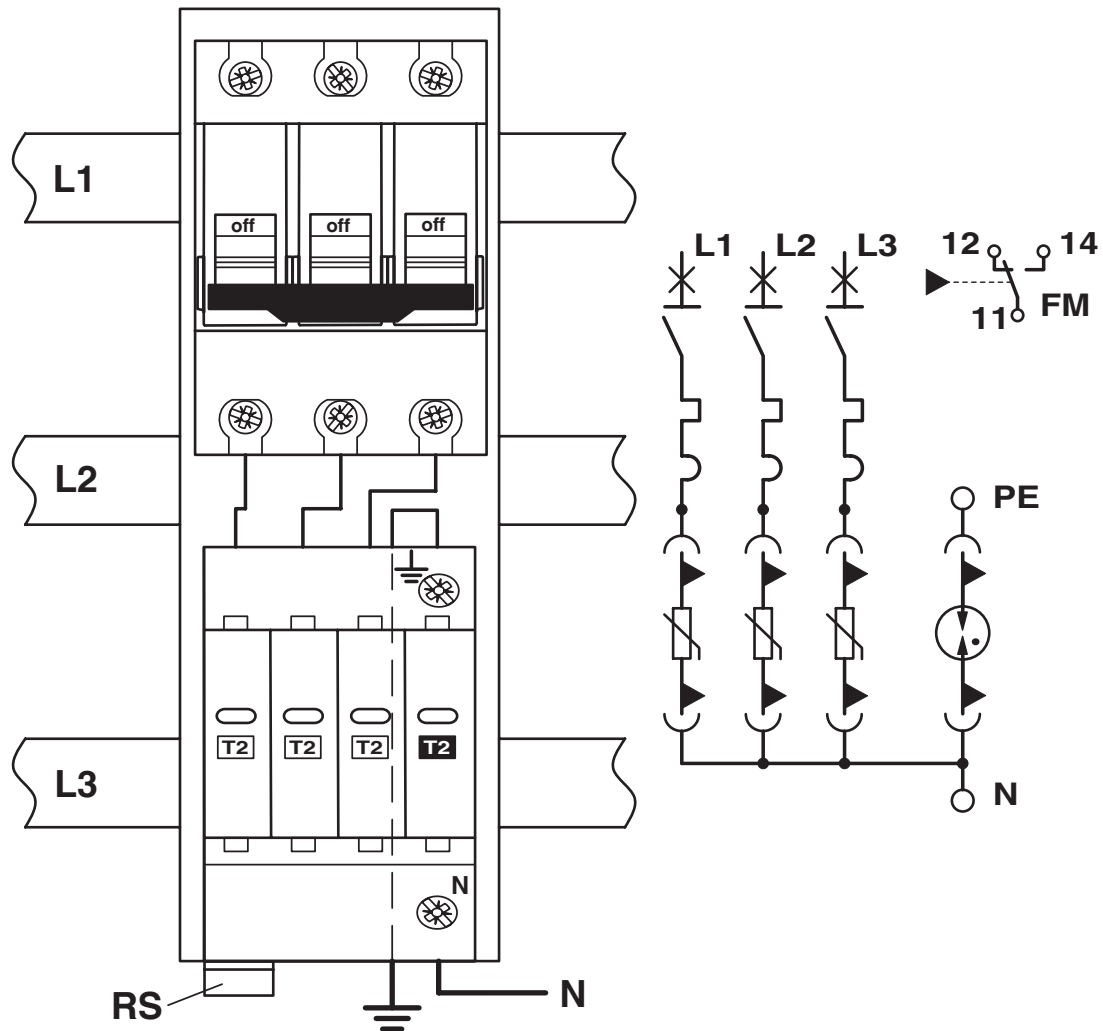
Application drawing
