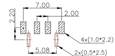
PCB.WELDING DRAWING (TOLERANCE:±0.05)
