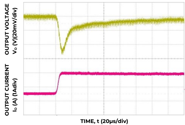
Figure 22. Transient Response to Dynamic Load Change from 50% to 100% at 12V in , C out =2x47μF, C Tune =2700pF, R Tune =267
