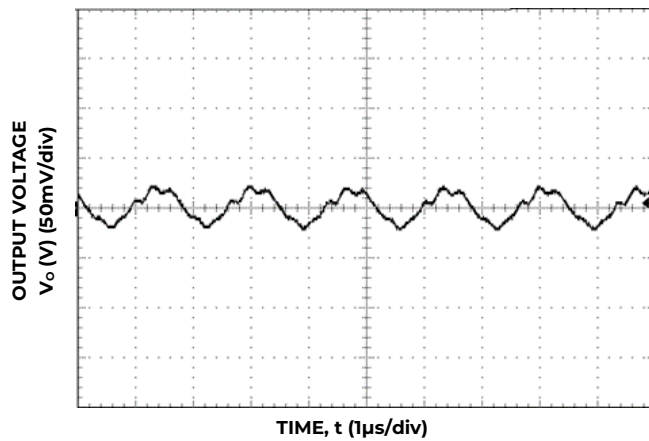
Figure 33. Typical output ripple and noise (C o =10μF ceramic, V IN = 12V, I o = I o,max ).
