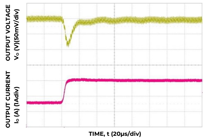
Figure 34. Transient Response to Dynamic Load Change from 50% to 100% at 12V in , C out =1x47μF, C Tune =820pF & R Tune =267
