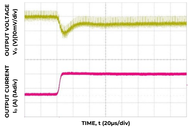
Figure 4. Transient Response to Dynamic Load Change from 50% to 100% at 12V in , C out =1x47μF+2x330μF, C Tune =27nF, R Tune =180
