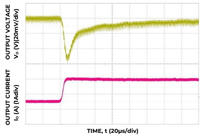
Figure 28. Transient Response to Dynamic Load Change from 50% to 100% at 12V in , C out =2x47μF, C Tune =2200pF, R Tune =267
