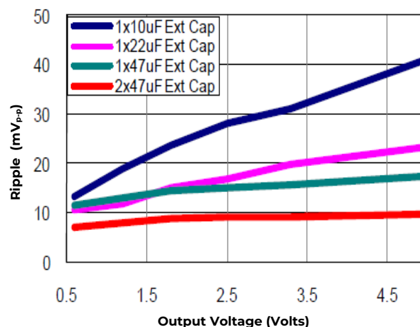
Figure 38. Output ripple voltage for various output voltages with external 1x10 \mu F, 1x22 \mu F, 1x47 \mu F or 2x47 \mu F ceramic capacitors at the output (3A load). Input voltage is 12V.
