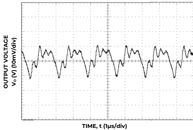
Figure 15. Typical output ripple and noise (C o =10μF ceramic, V IN = 12V, I o = I o,max ).
