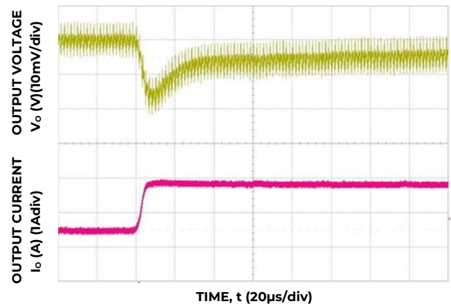
Figure 10. Transient Response to Dynamic Load Change from 50% to 100% at 12V in , C out =1x47μF+1x330μF, C Tune =10nF, R Tune =267
