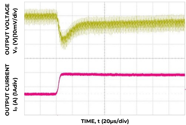
Figure 16. Transient Response to Dynamic Load Change from 50% to 100% at 12V in , C out =1x47μF+1x330μF, C Tune =10nF & R Tune =267
