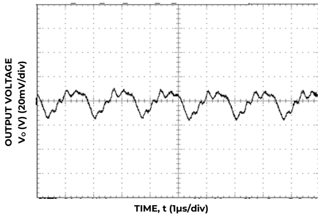
Figure 21. Typical output ripple and noise (C o =10μF ceramic, V IN = 12V, I o = I o,max ).
