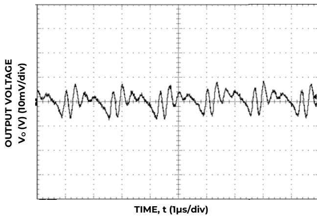
Figure 3. Typical output ripple and noise (C O =10μF ceramic, V IN = 12V, I o = I o,max ).
