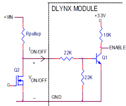
Figure 40. Circuit configuration for using negative On/Off logic.
