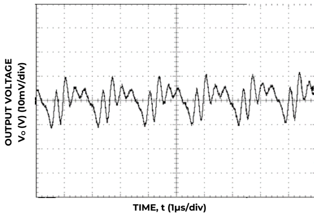
Figure 9. Typical output ripple and noise (C O =10μF ceramic, V IN = 12V, I o = I o,max ).
