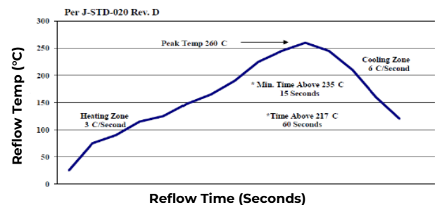
Figure 51. Recommended linear reflow profile using Sn/Ag/Cu solder.
