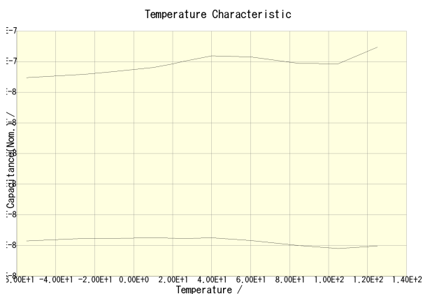
C3216X7R2E104K160AA(DC Bias = 0V) C3216X7R2E104K160AA(DC Bias = 125V)
