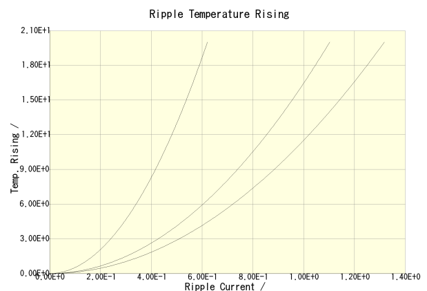
C3216X7R2E104K160AA(100kHz) C3216X7R2E104K160AA(500kHz) C3216X7R2E104K160AA(1MHz)
