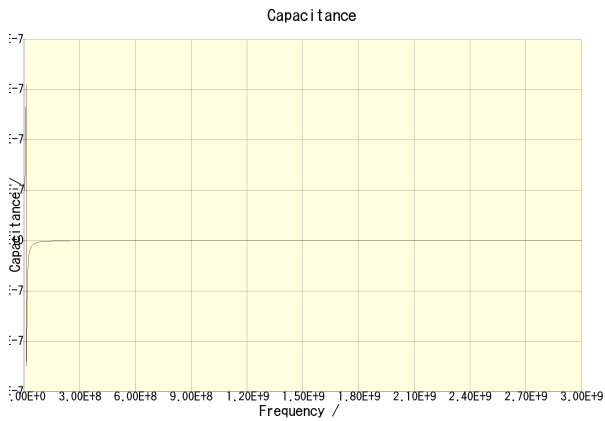
C3216X7R2E104K160AA
