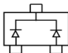
MMBD 4148 CCX MARKING:D5
