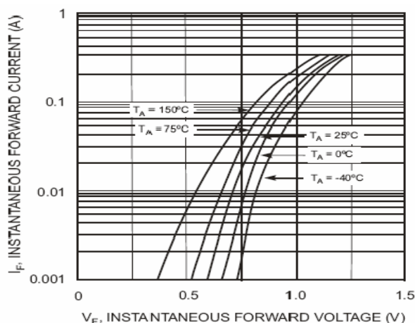
Fig. 2 Forward Characteristics
