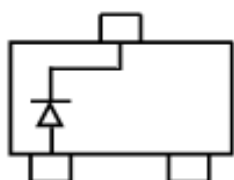
MMBD 4148 AX MARKING:5H
