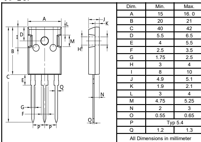
TO-247
