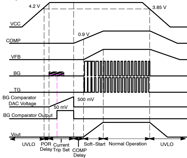
Figure 18. Soft-Start Sequence
