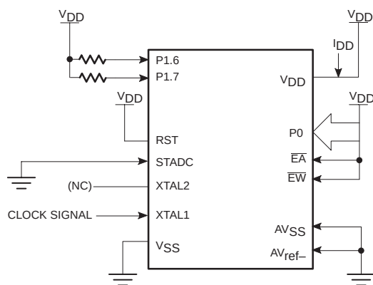
Figure 58. I_{DD} Test Condition, Active Mode All other pins are disconnected 1
