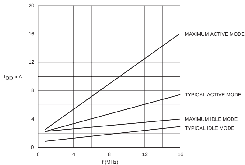
Figure 57. 16 MHz Version Supply Current ( I_{DD} ) as a Function of Frequency at XTAL1 ( f_{osc} )
