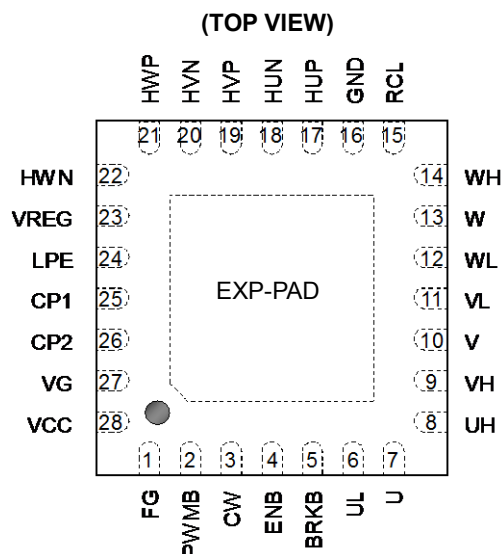
Figure 2. Pin Configuration
