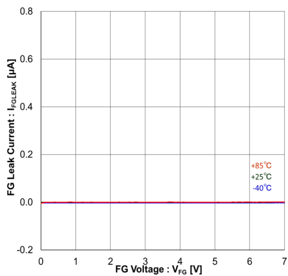
Figure 12. FG Leak Current vs FG Voltage
