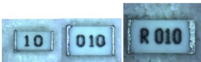
Fig 1. Construction of 0603/0805/1206
