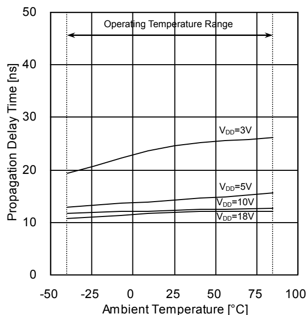
Figure 12. Propagation Delay Time IN→OUT( t_{PLH} ) vs Ambient Temperature
