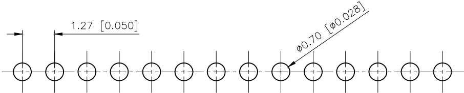
PCB LAYOUT
