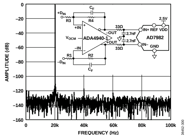
Figure 2. ADA4940-1 Driving the AD7982 ADC
