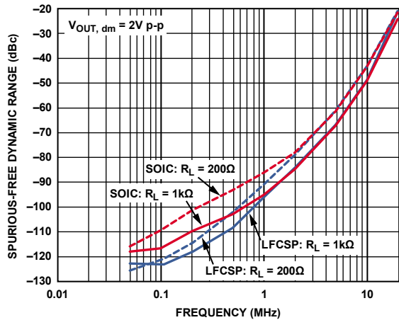
Figure 31. Spurious-Free Dynamic Range vs. Frequency at R_L = 200\ \Omega and R_L = 1\text{ k}\Omega
