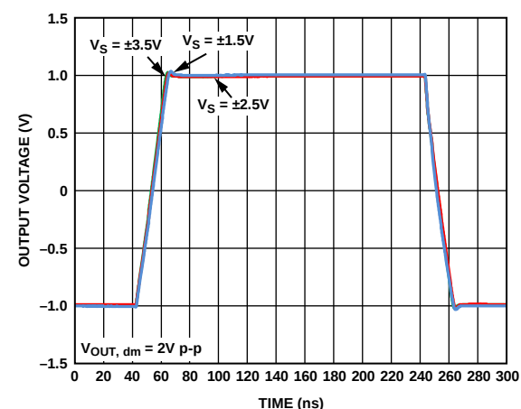
Figure 53. Large Signal Transient Response for Various Supplies
