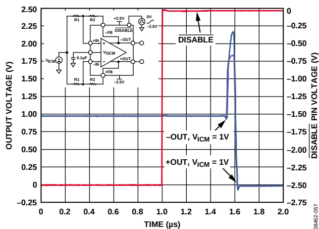
Figure 48. \overline{DISABLE} Pin Turn-On Time
