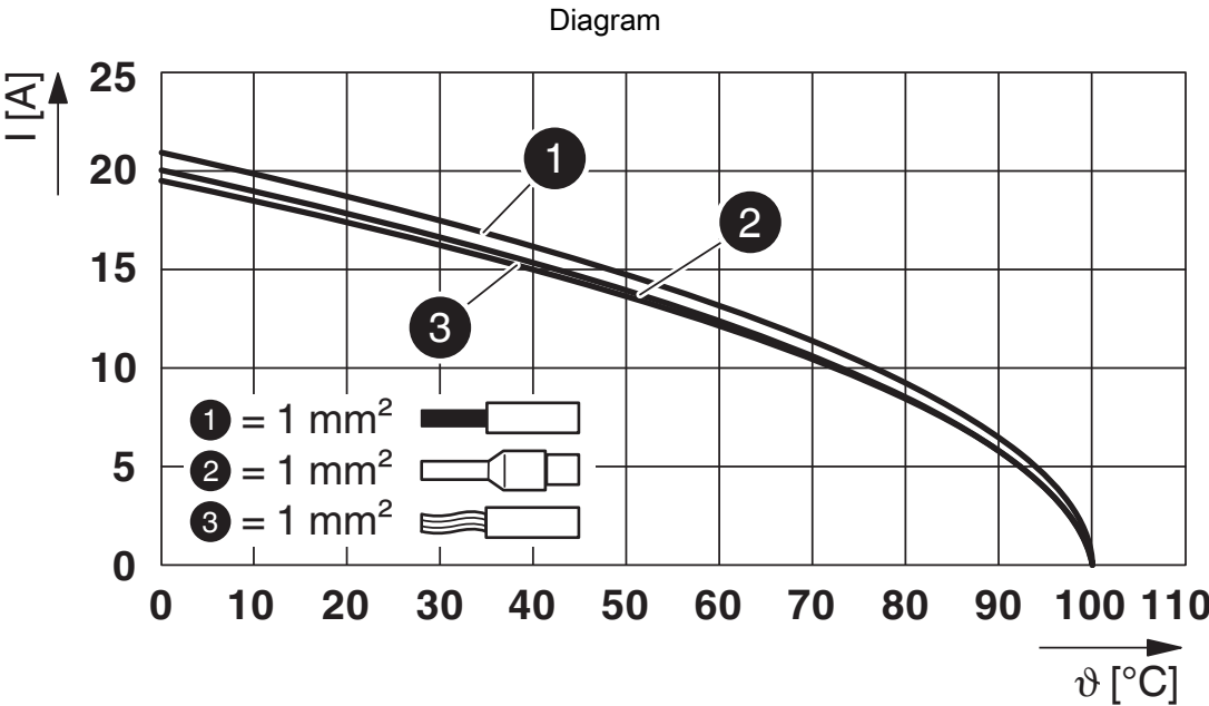
Derating diagram for 1.0 mm 2
