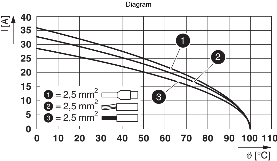
Derating diagram for 2.5 mm 2
